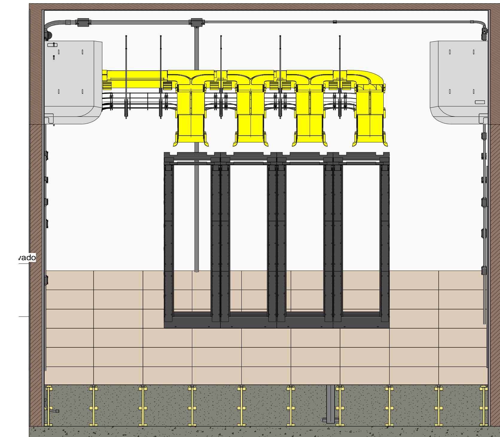
5 3D - TELECOM 1
