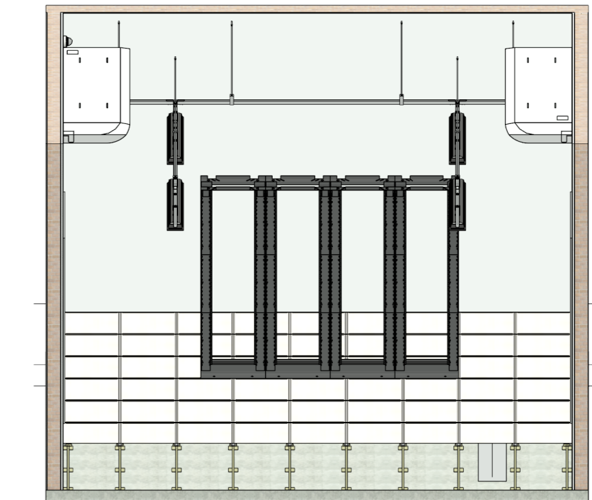
5 3D - TELECOM 1
